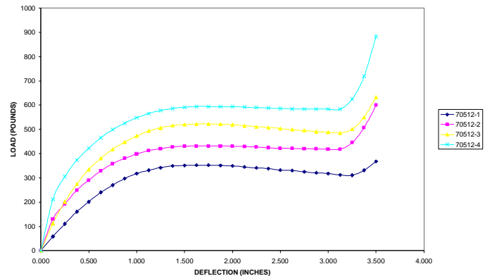
LOAD VS. DEFLECTION (RADIAL)
