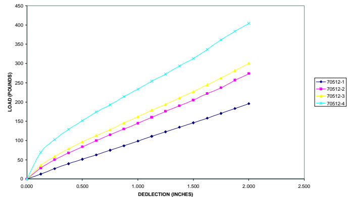
LOAD VS. DEFLECTION (RADIAL)
